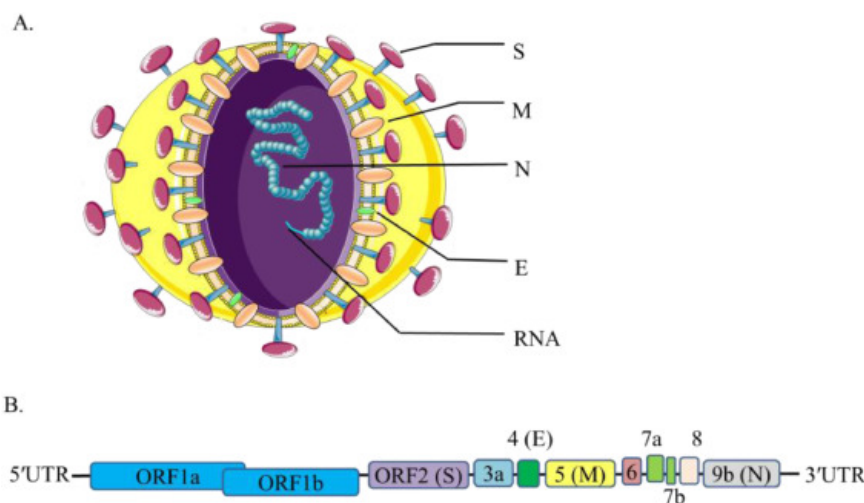
Figure 1. SARS CoV-2 genome organization with following gene order: 5'-replicase (ORF1ab)-structural proteins [S-E-M-N]-3'
